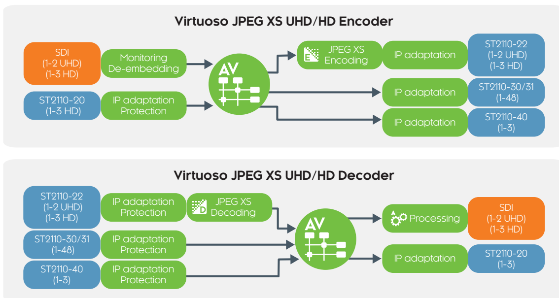
Functional diagram (HBR 10G)
