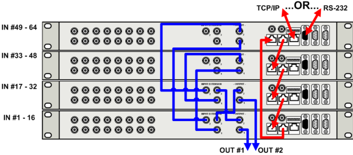
Figure 10: SL-AD6402-75 wiring diagram.
