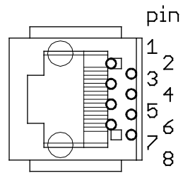
Figure 6: Pin layout 8P8C Modular jack
